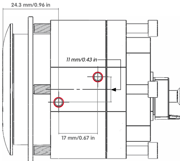
Drilling template for screws at the bottom
