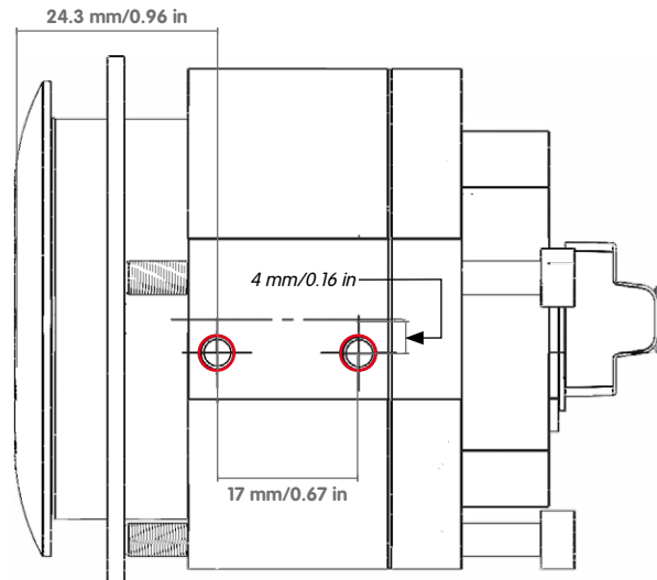
Drilling template for screws at the side
